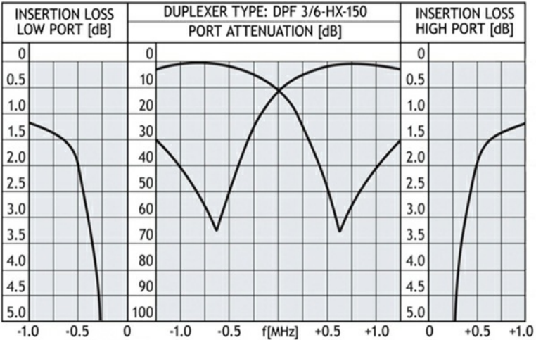
TYPICAL RESPONSE CURVE @ 1.3 MHz DUPLEX SPACING
